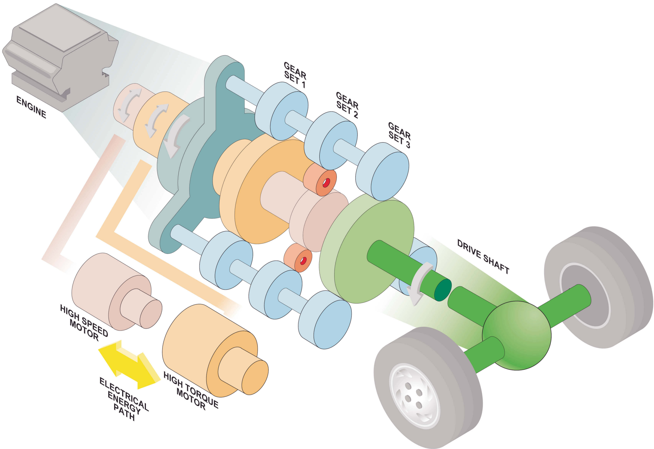
The shafts of the light blue planet gears move around the sun as the planets rotate on their own axis. The two electric motors are on the two suns. The orange motor is on the left-hand sun, the brown motor is on the middle sun, and the output is on the green sun. The input from the grey engine is on the dark green carrier. The light blue planets are all connected together.
